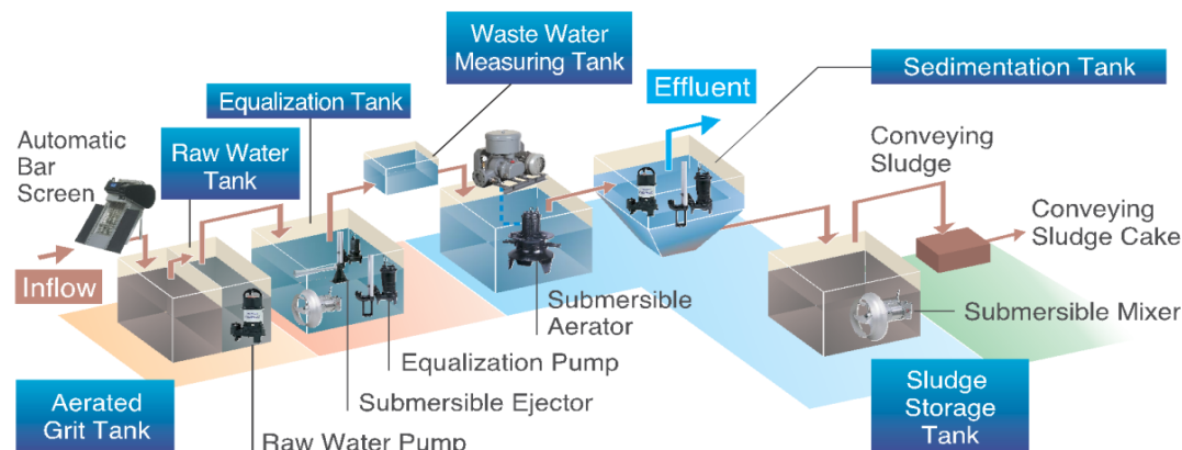
Variety line up of wastewater treatment equipment
